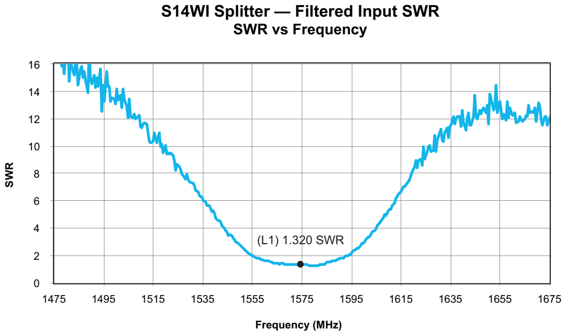
Figure 2-8. Filtered Input SWR
