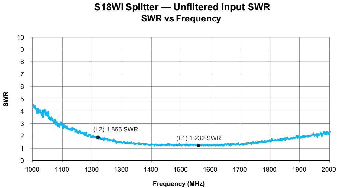
Figure 2-2. Unfiltered Input SWR
