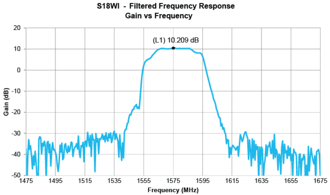
Figure 2-7. Frequency Filtered Response
