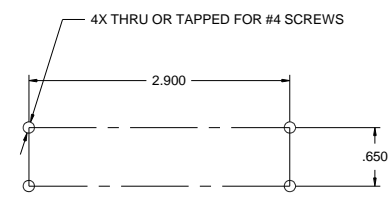
RECOMMENDED MOUNTING PATTERN
