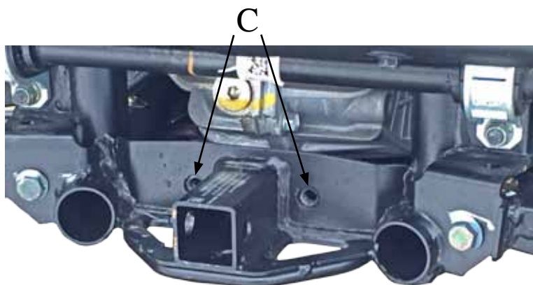
Factory 1 1/4" Receiver / 2" Mount location
