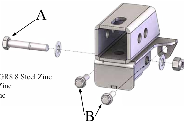
“Figure 1” Exploded View
