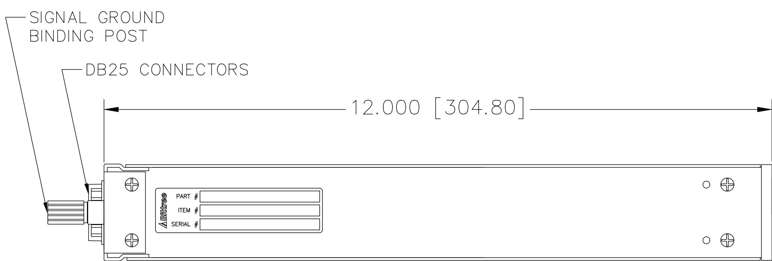
LEFT VIEW
