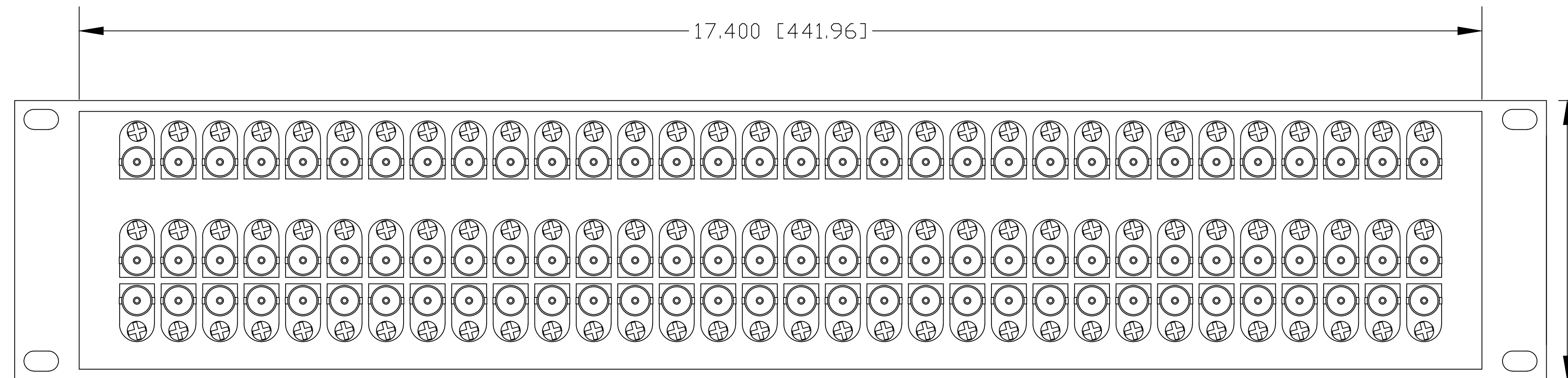
REAR VIEW
