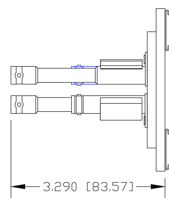
SIDE VIEW
