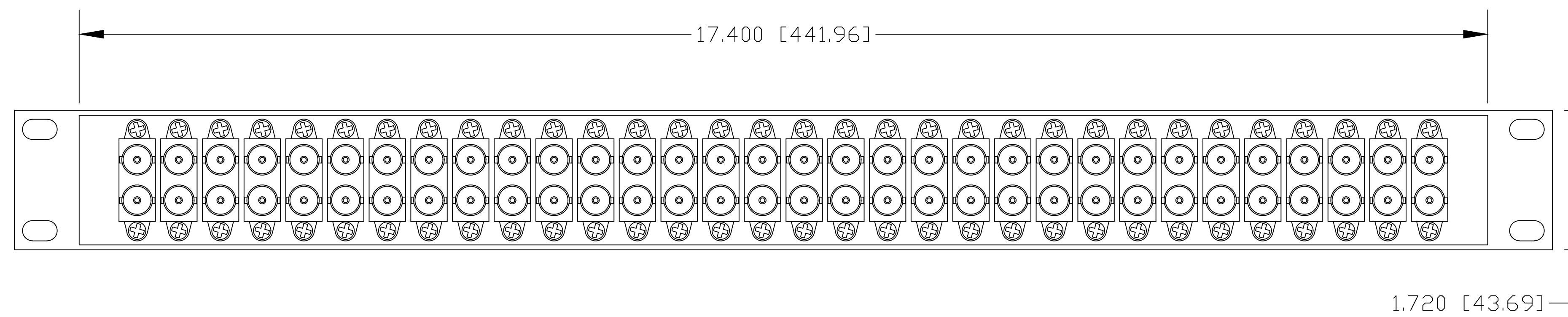
REAR VIEW
