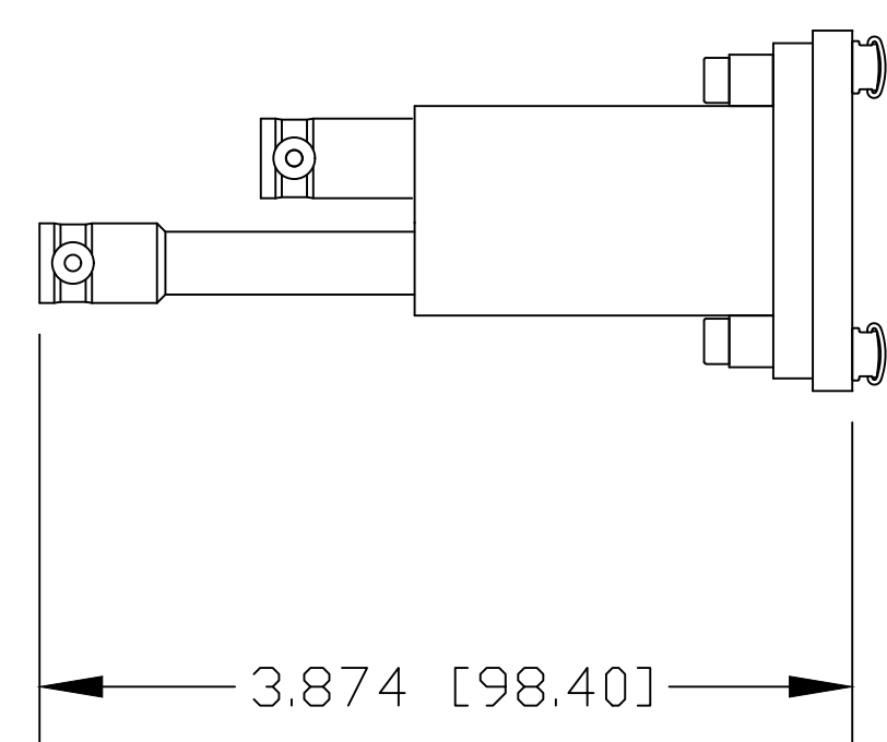
SIDE VIEW
