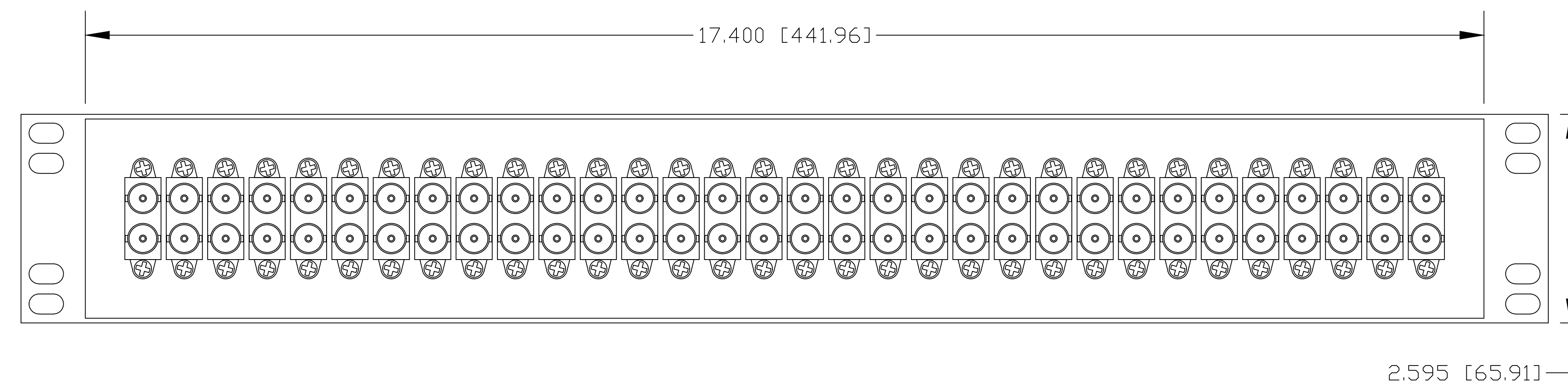
REAR VIEW
