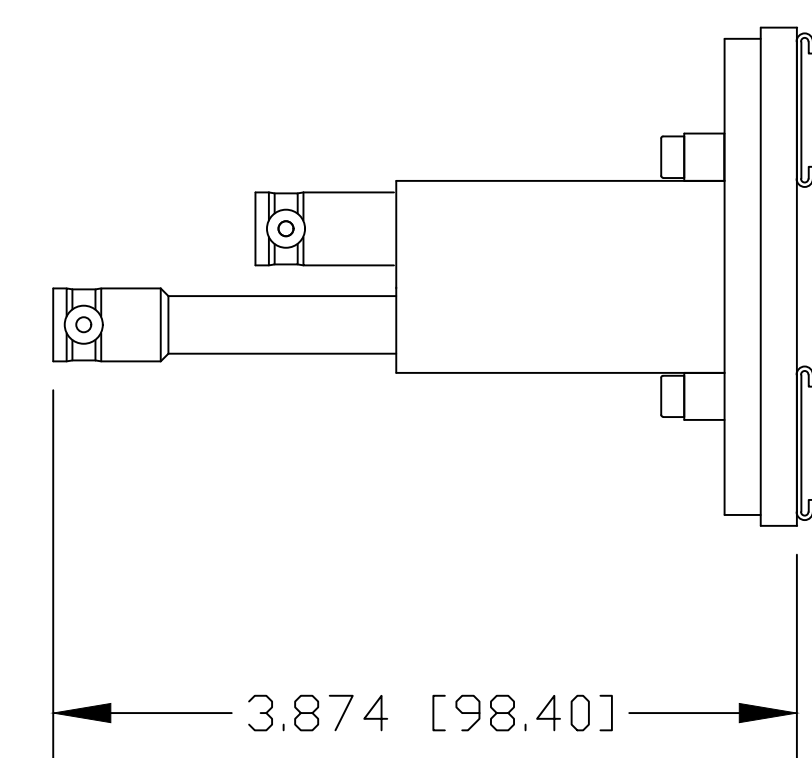
SIDE VIEW
