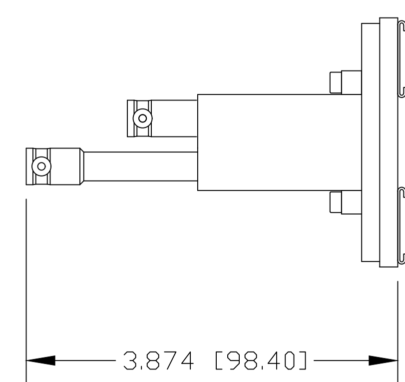
SIDE VIEW
