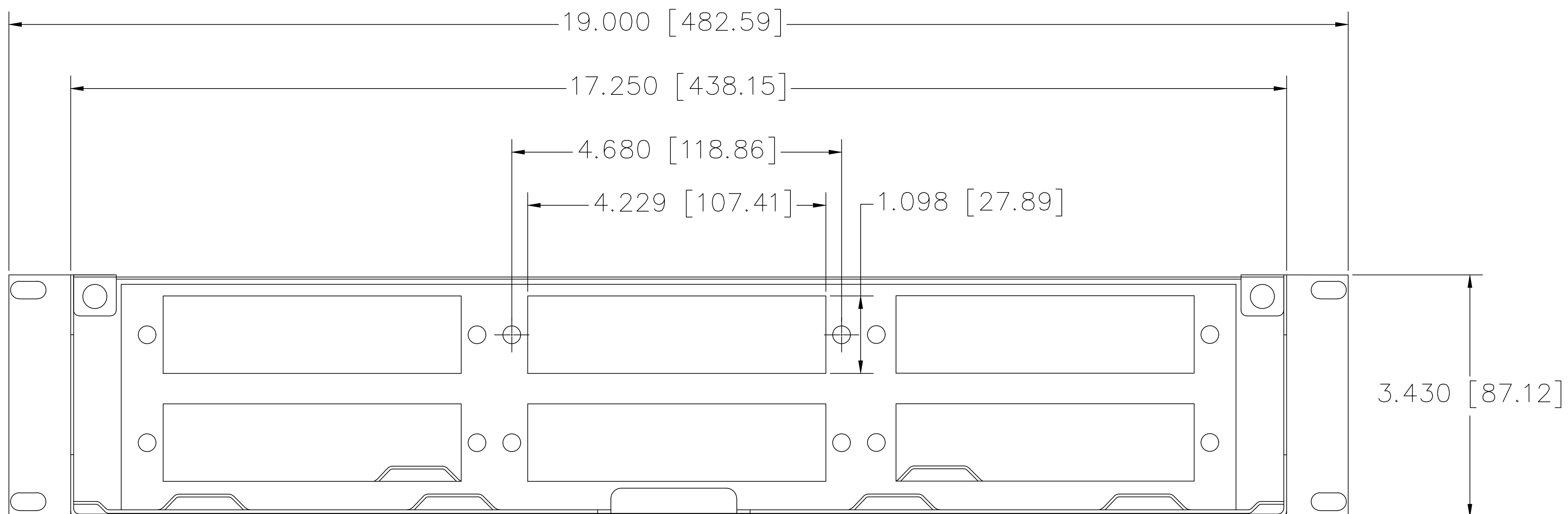
FRONT VIEW
