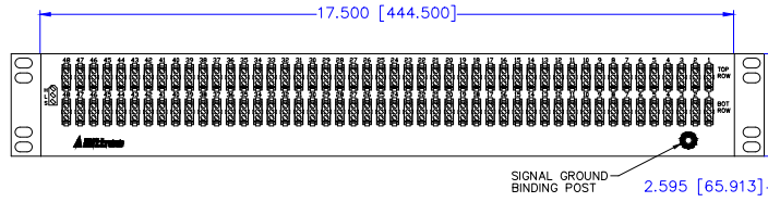
REAR VIEW
