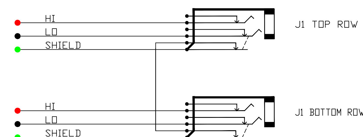
SCHMATIC NON-NORMALED SWITCHED GND VIEW
