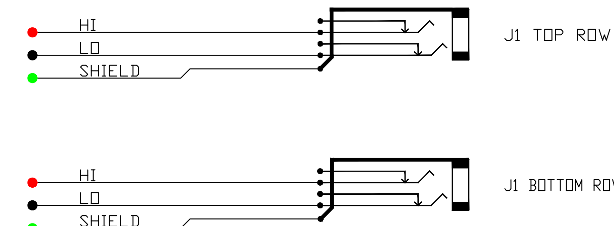
SCHEMATIC NON-NORMALED ISOLATED GND VIEW
