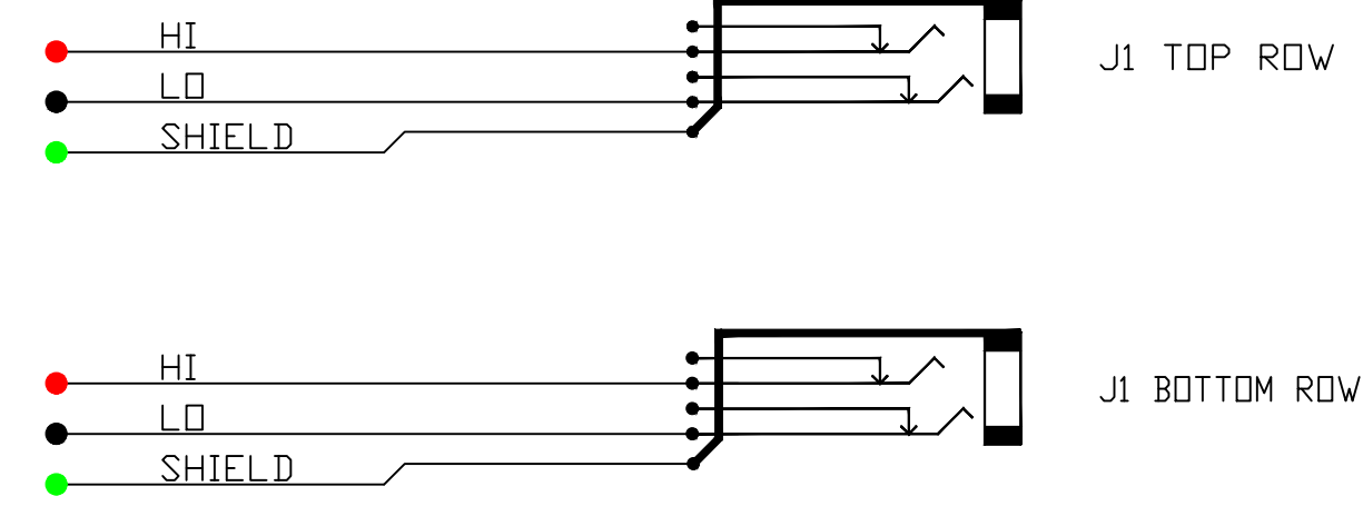
SCHEMATIC NON-NORMALIZED ISOLATED GND VIEW
