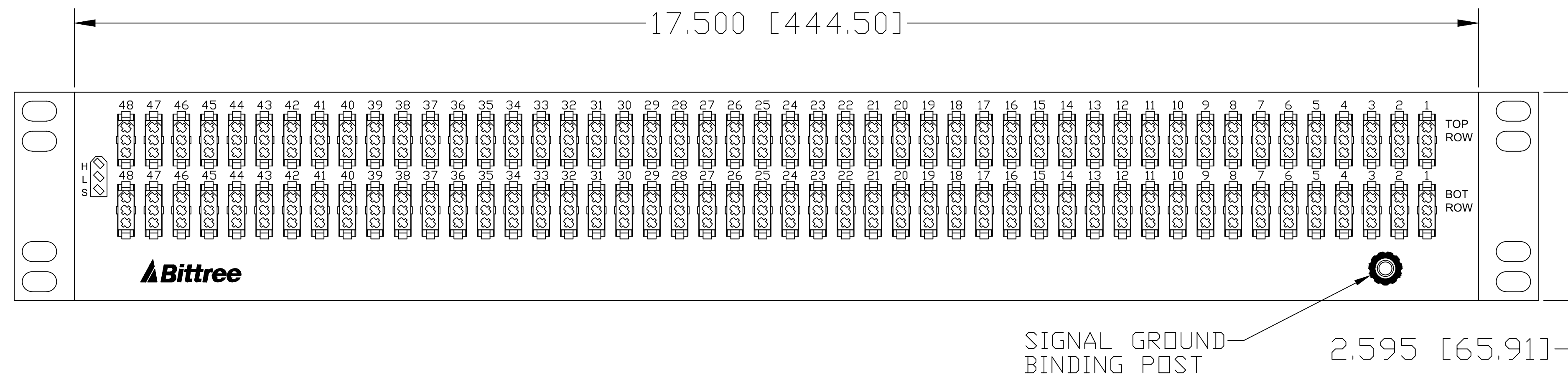
REAR VIEW
