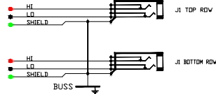
SCHEMATIC NON-NORMALED BUSSED GND VIEW
