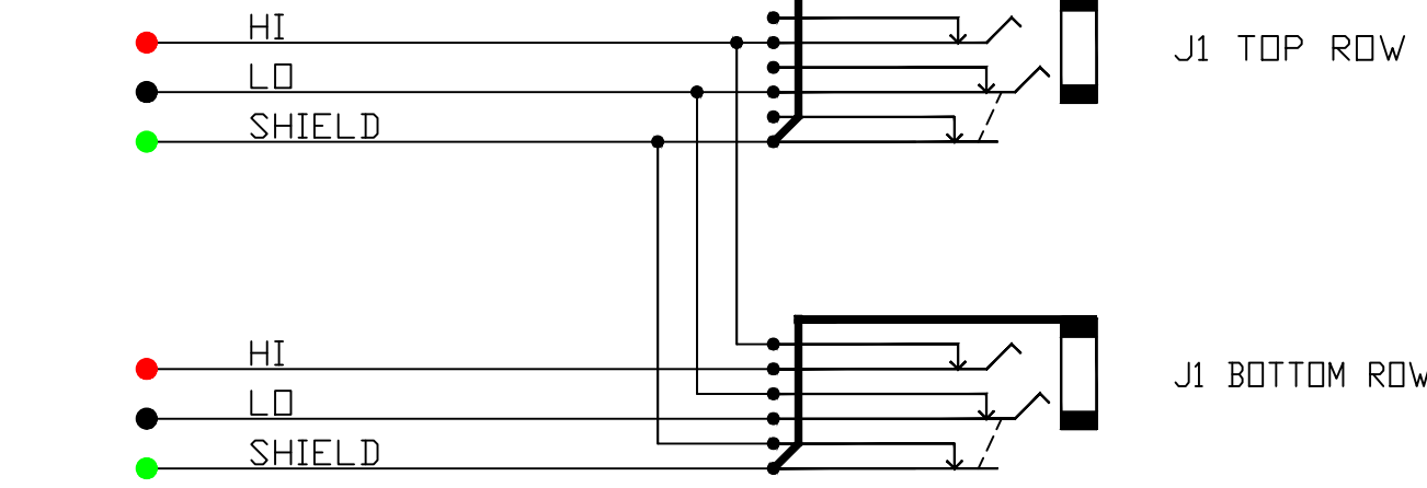
SCHEMATIC HALF-NORMALIZED SWITCHED GND VIEW
