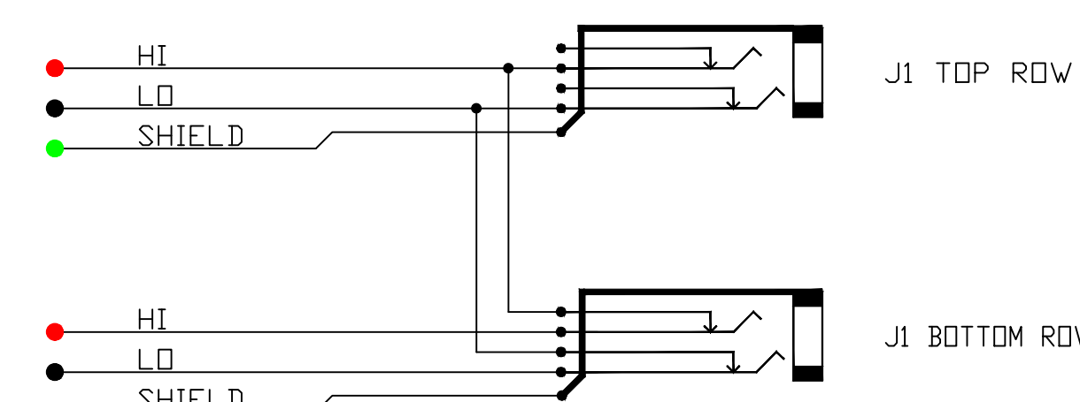
SCHMATIC HALF-NORMALED ISOLATED GND VIEW
