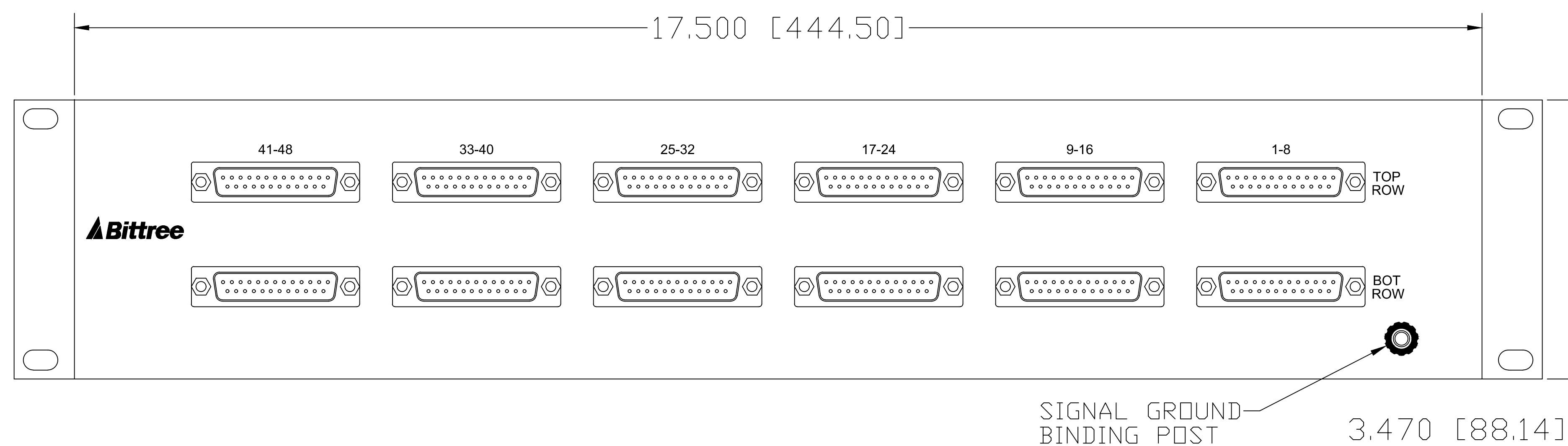
REAR VIEW
