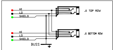
SCHEMATIC HALF-NORMALED BUSSED GND VIEW
