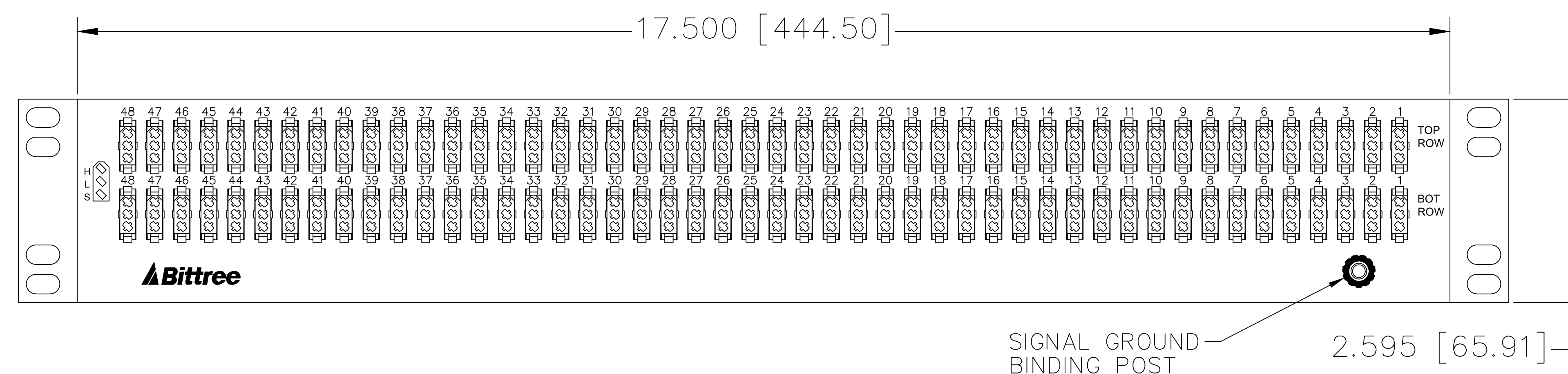
REAR VIEW
