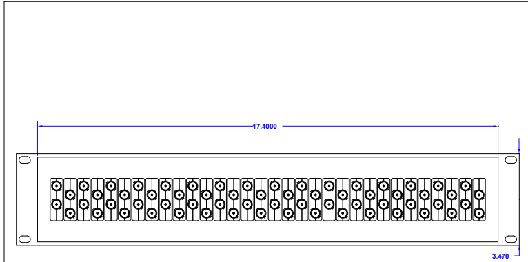
REAR VIEW
