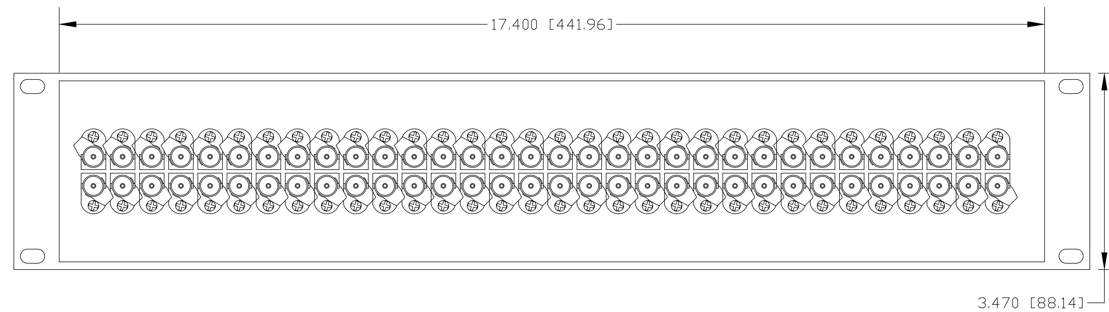
REAR VIEW
