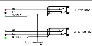
SCHEMATIC NON-NORMALED BUSSED GND VIEW
