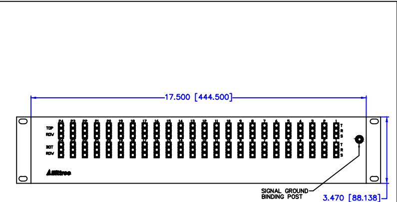
REAR VIEW
