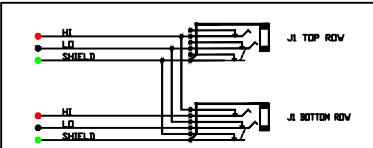
SCHEMATIC HALF-NORMALIZED SWITCHED GND VIEW
