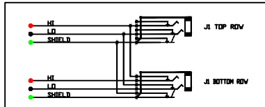
SCHEMATIC HALF-NORMALIZED SWITCHED GND VIEW
