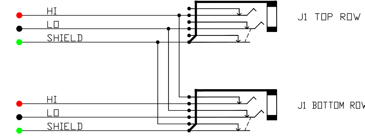
SCHEMATIC HALF-NORMALIZED SWITCHED GND VIEW
