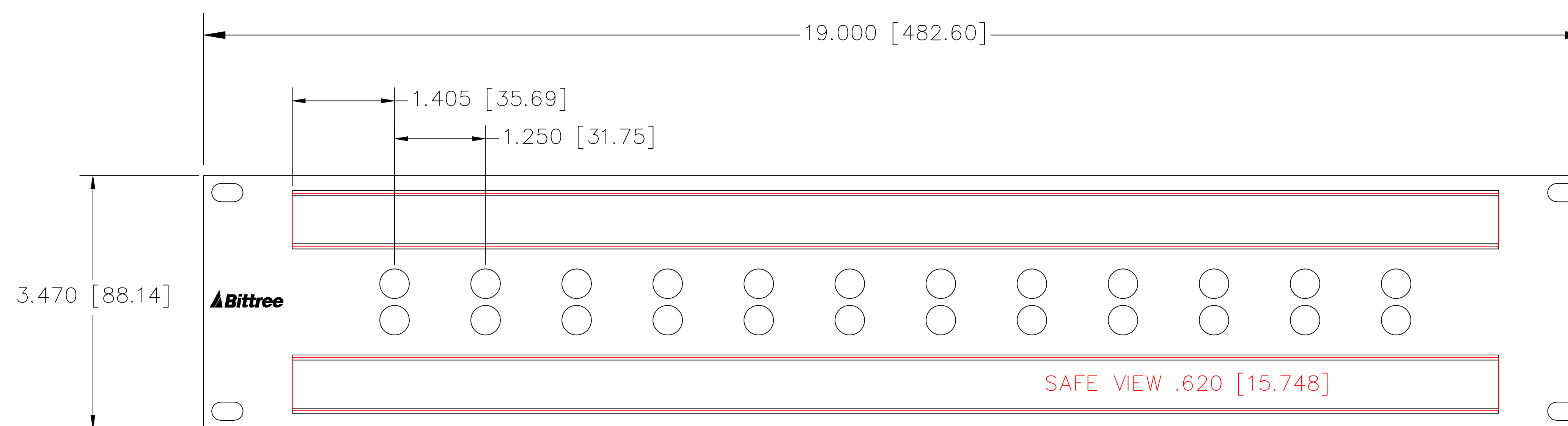
FRONT VIEW
