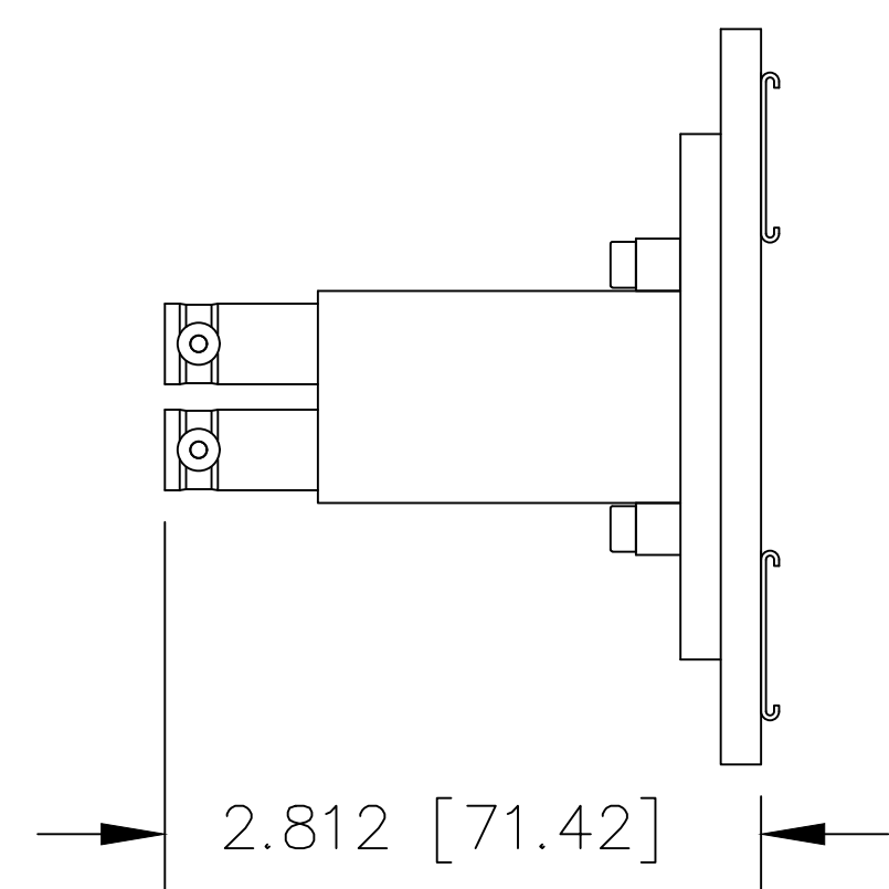
SIDE VIEW
