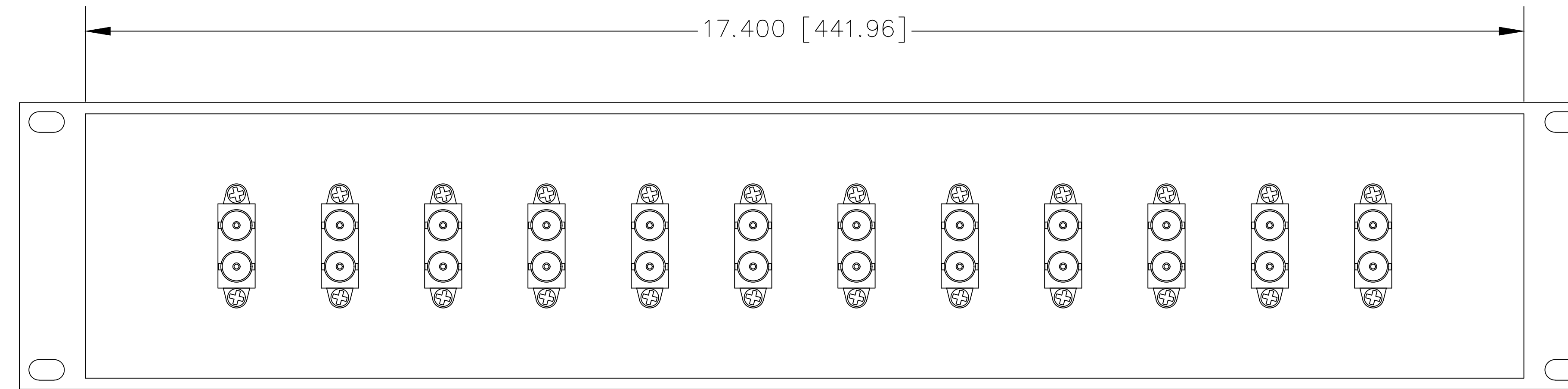
REAR VIEW
