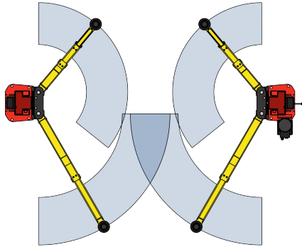
SYMMETRIC INSTALLATION
