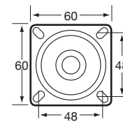
NNN40/NZPBR Plate with swivel and wheel brake
