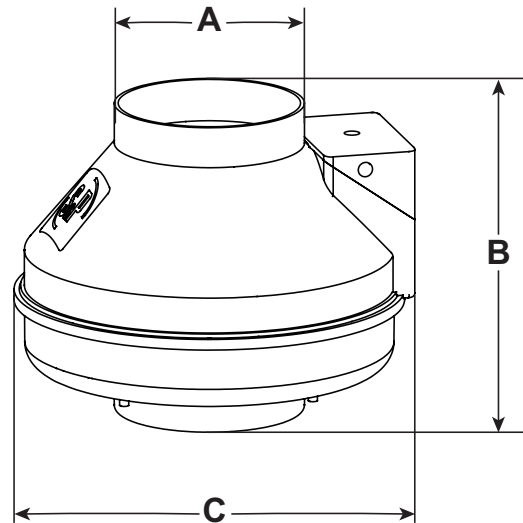
PRF-150 Dimensions
