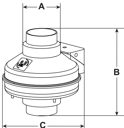
PRF-100 Dimensions
