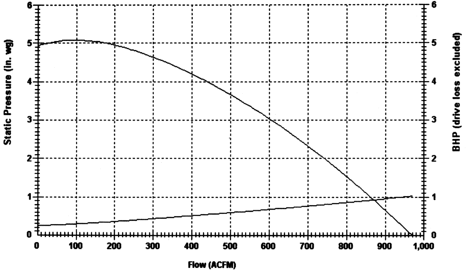
HADP12-1 WITH 11 x 2-3/4" WHEEL @ 2700 RPM .075 lb/ft 3 DENSITY, 7.0 IN. INLET
