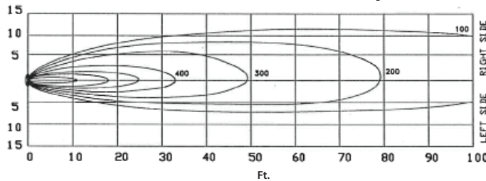
Airmaster 24HF36 Horizontal Velocity Profile
