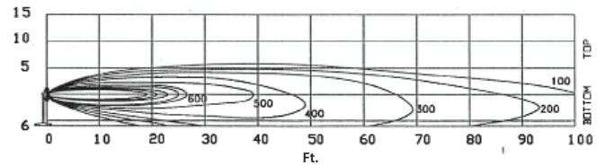
Airmaster 30HF36 Vertical Velocity Profile
