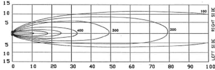
Airmaster 24HF36 Vertical Velocity Profile
