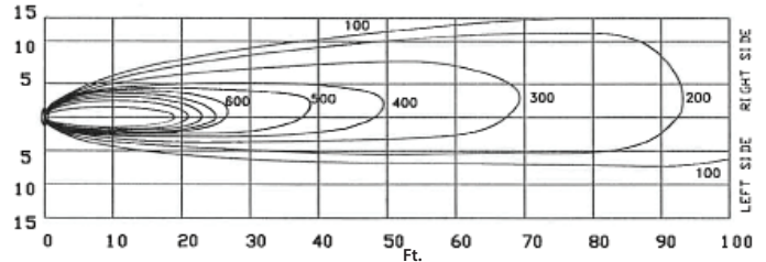
Airmaster 30HF36 Horizontal Velocity Profile
