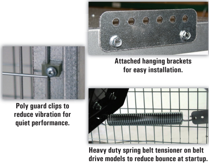
Shown: Back of 36" Belt Drive, Galvanized 4 Blade Whirl-Wind
