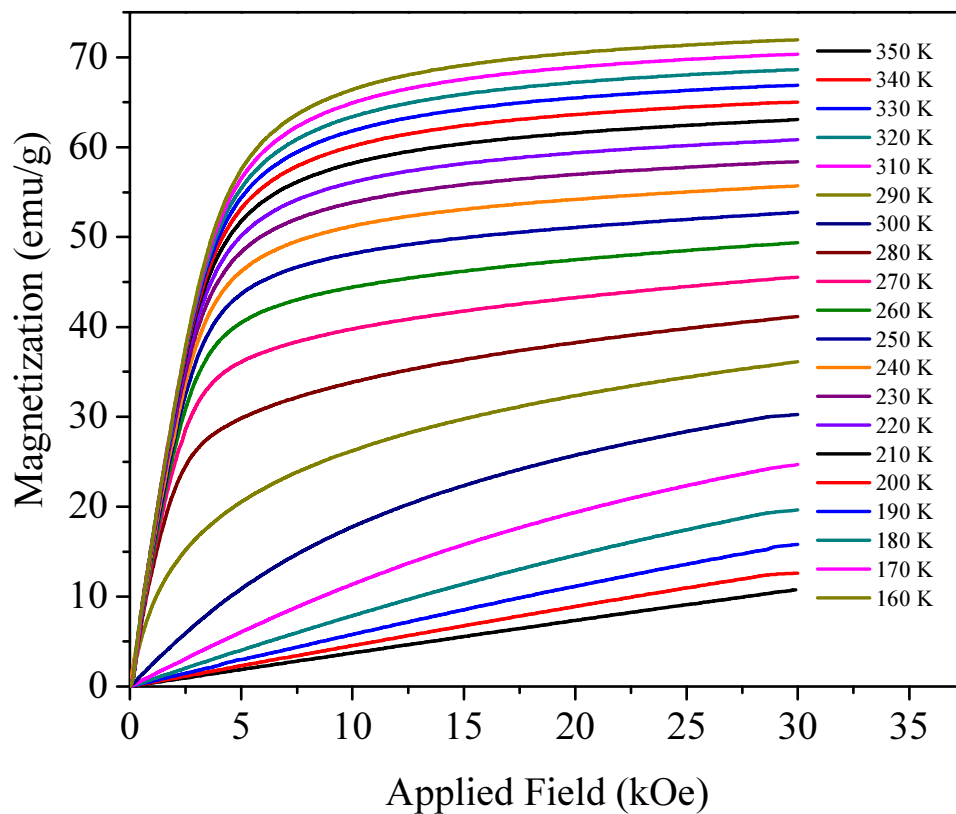
Gadolinium Isothermal Curves
