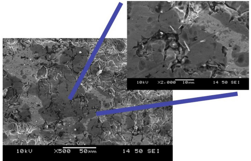
Fig 4. Scanning electron micrographs to demonstrate the uneven nature of surfaces that need to be disinfected. Shown here is stainless steel; due to their small size (bacteria are often less than 1 \mu\text{m} in diameter) cells inside these micro-crevices are often out of reach of mechanical removal as well as chemicals applied to the surface. Nano-technology, including 'smart materials' with inherent antimicrobial properties and protective antimicrobial coatings show much promise in this regard as they prevent the establishment of bacterial micro-colonies.
