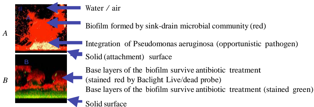
Fig 2. Cross sections of biofilms performed with scanning confocal laser microscopy showing (A) that environmental biofilms provide a habitat for pathogens to proliferate, and (B) where they show notable protection against antimicrobials.
