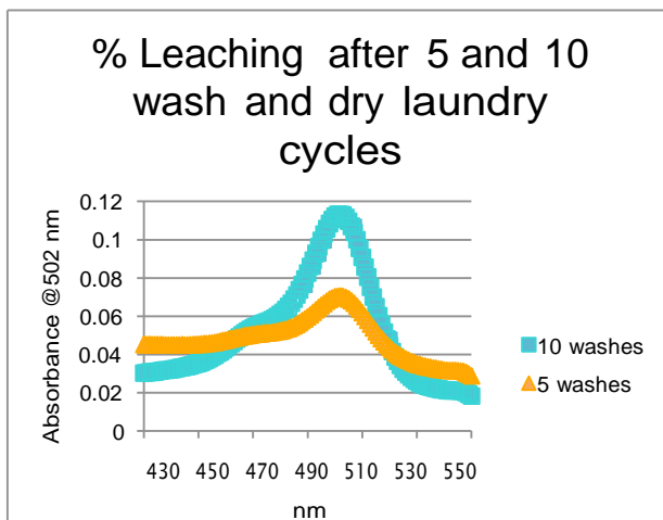
Fig 8. EV360™ showed remarkable binding strength and stability even after repeated wash cycles in an industrial laundry facility. The percentage loss of the molecule was calculated to be on average 0.106% / wash cycle or 0.53% after 10 cycles.
