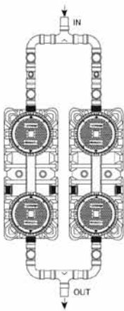
2 no. XL100 – PARALLEL Up to 200GPM, 2116 lbs Grease Capacity.
