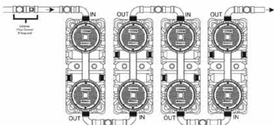
4 no. XL100 – PARALLEL - Up to 400GPM, 4232 lbs Grease Capacity.
