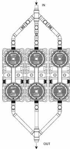
3 no. XL100 – PARALLEL Up to 300GPM, 3174 lbs Grease Capacity.
