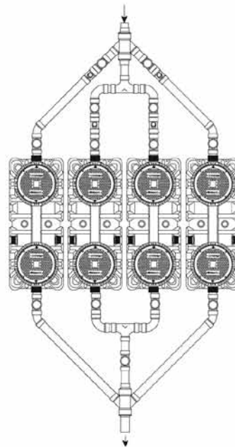
4 no. XL100 – PARALLEL Up to 400GPM, 4232 lbs Grease Capacity.
