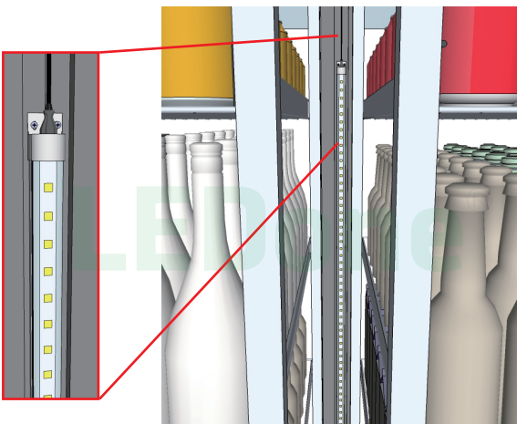
3. The side installation drawing (look from the fridge behind)
