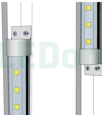
(Screwed to the top and bottom)
