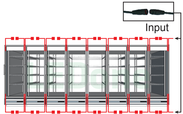
2. The installation instruction for LED cooler light (can be installed upside and down side)
