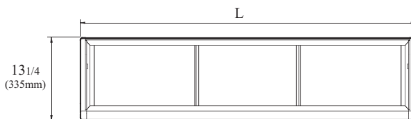
TOMD-L : Front View
