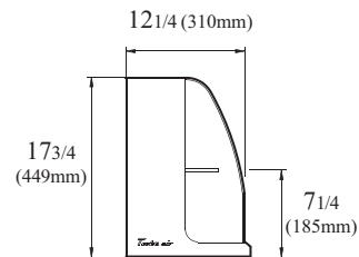
TOMD-H : Side View
