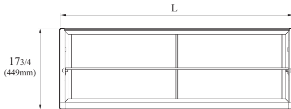
TOMD-H : Front View
