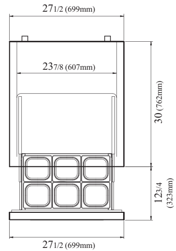
PLAN VIEW
