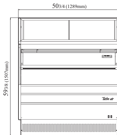
FRONT VIEW (W/ TOMD)
