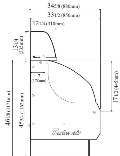
SIDE VIEW (W/ TOMD)
