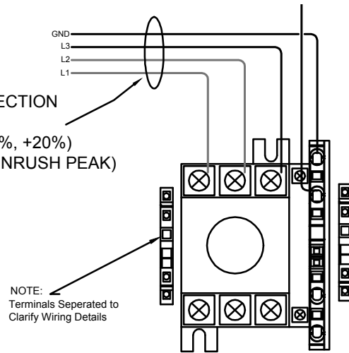
FIGURE 10C THREE PHASE
