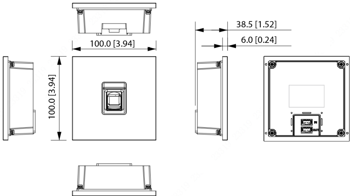
Figure 3-1 Dimensions (unit: mm [inch])
