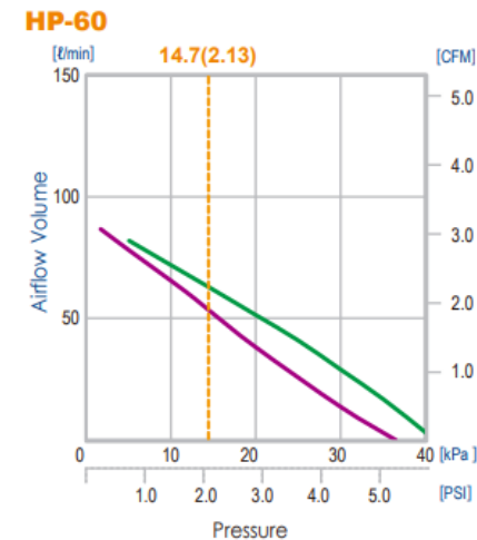
Performance Curves
