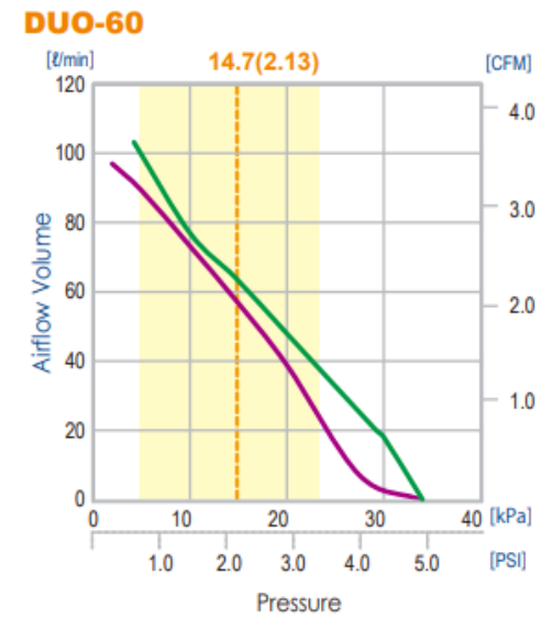
Performance Curves
