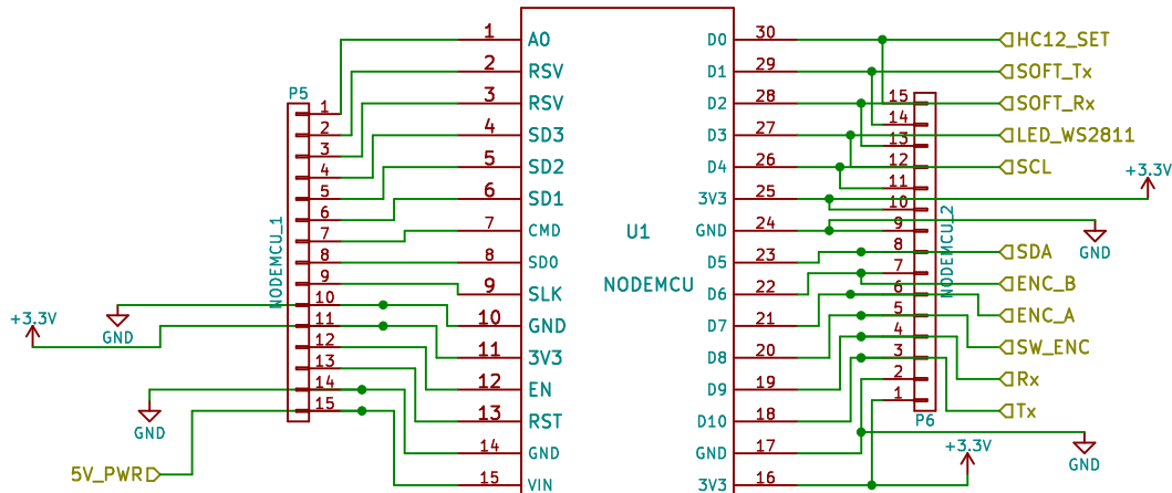
800mA 3.3V regulator on NodeMCU
