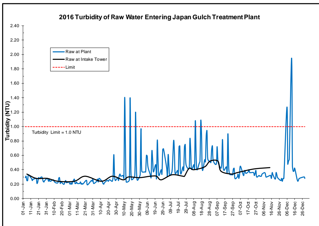
Figure 8 2016 Turbidity of Raw Water Entering Japan Gulch Treatment Plant
