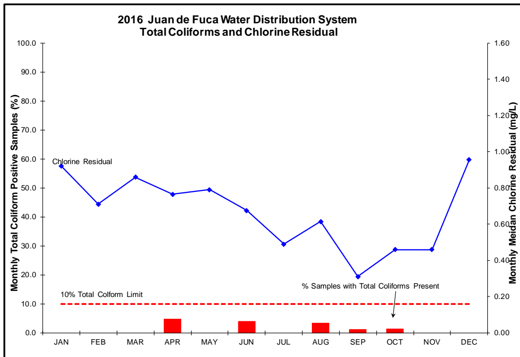
Figure 20 JDF – West Shore Distribution System Total Coliforms and Chlorine Residual
