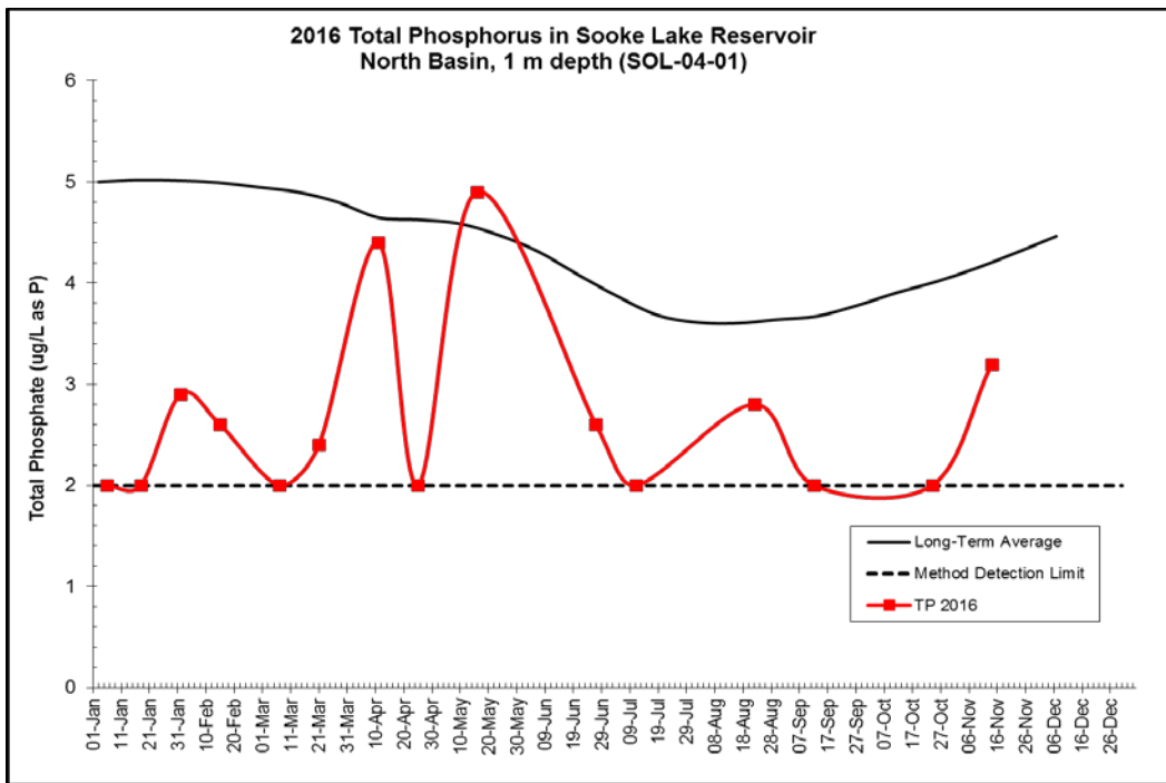
Figure 13 Total Phosphorus in Sooke Lake Reservoir, North Basin, 1 m depth (SOL-04-01)
