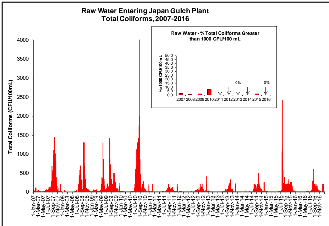
Figure 2 Raw Water Entering Japan Gulch Plant Total Coliforms 2007–2016
