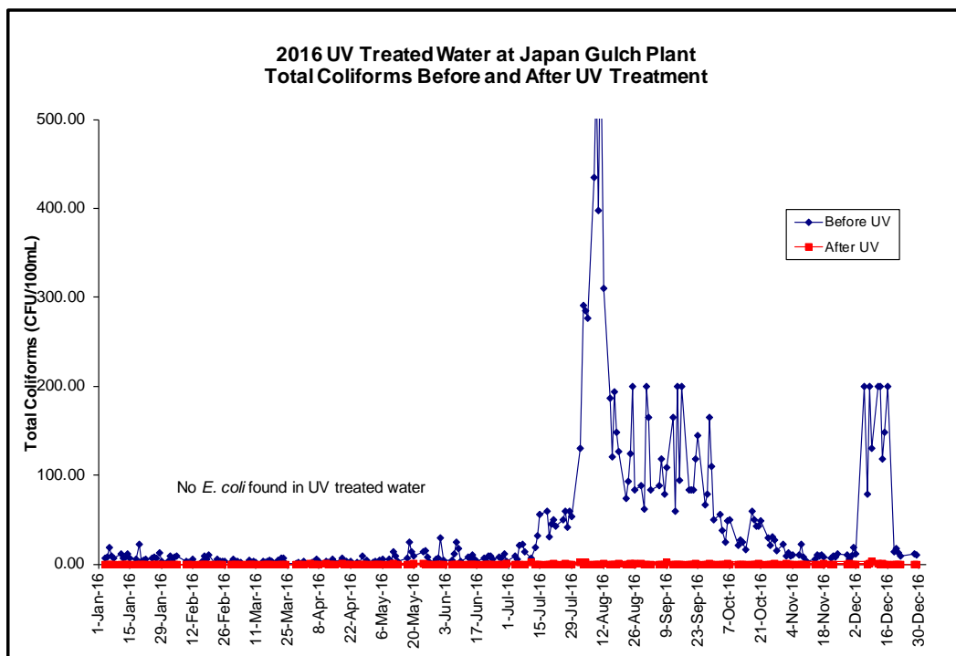
Figure 14 2016 UV Treated Water at Japan Gulch Plant Total Coliforms Before and After UV Treatment
