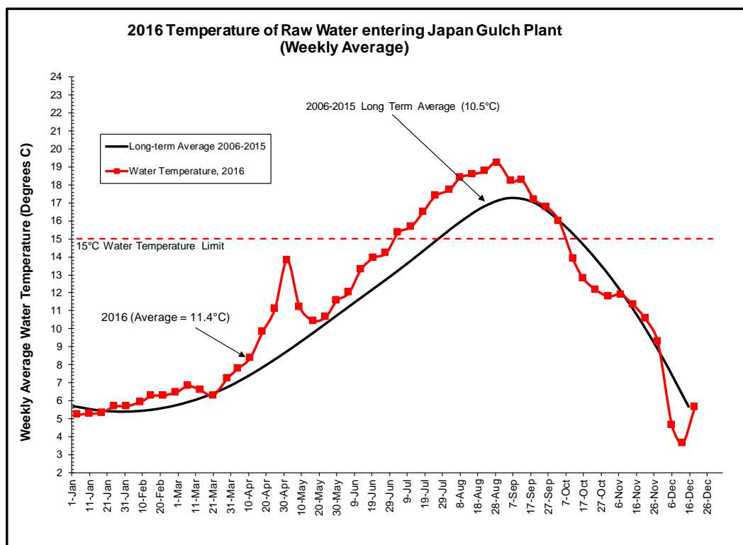
Figure 9 2016 Temperature of Raw Water Entering Japan Gulch Plant (Weekly Average)
