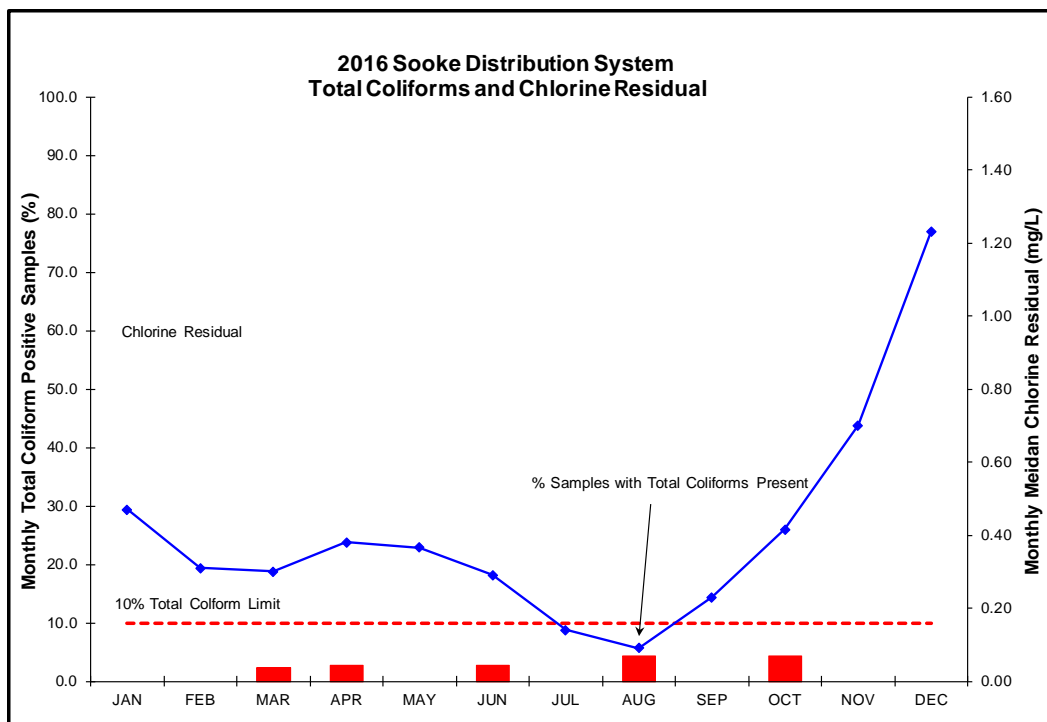
Figure 21 Sooke/East Sooke Distribution System Total Coliforms and Chlorine Residual
