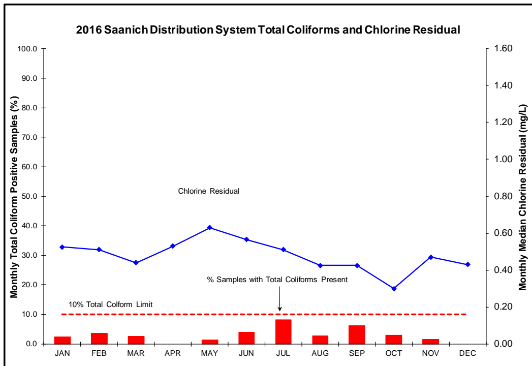
Figure 25 Saanich Distribution System Total Coliforms and Chlorine Residuals in 2016
