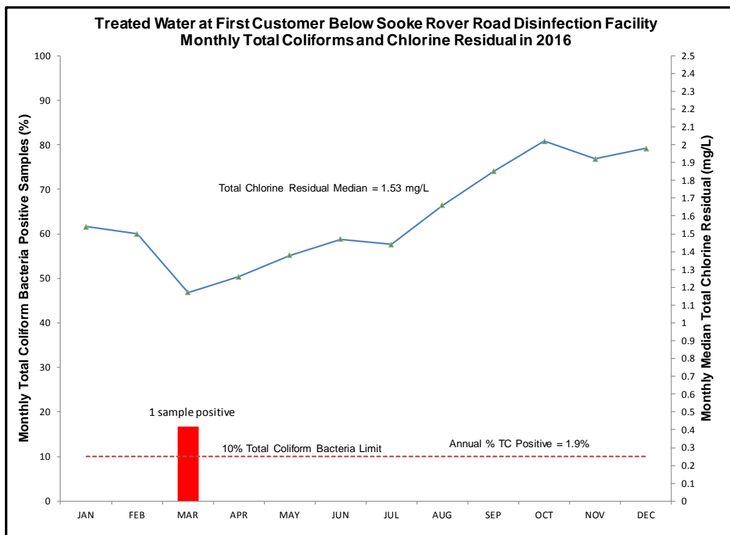
Figure 17 Treated Water at First Customer below Sooke Rover Road Disinfection Facility, Monthly Total Coliforms and Chlorine Residual in 2016
