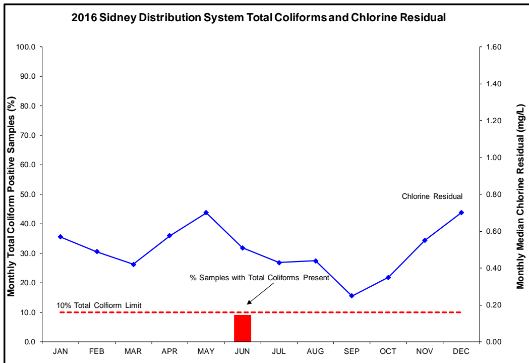
Figure 26 Sidney Distribution System Total Coliforms and Chlorine Residuals in 2016
