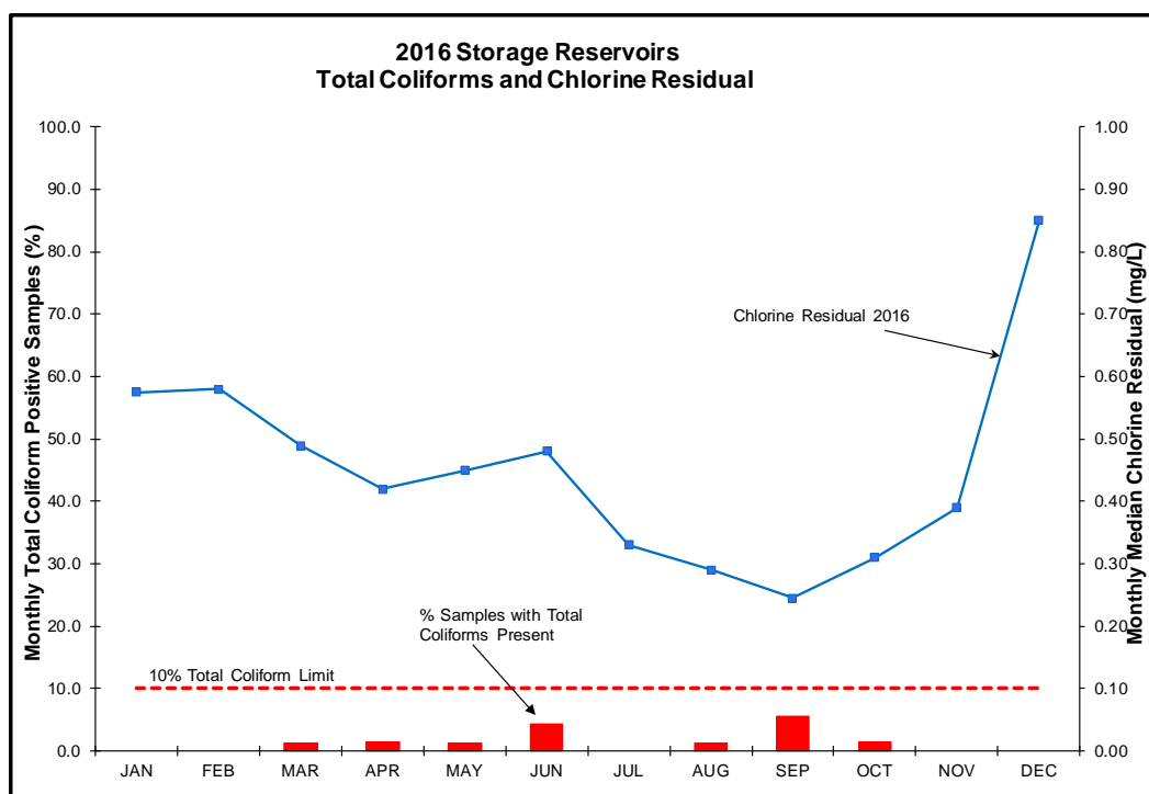
Figure 19 2016 Storage Reservoirs Total Coliforms and Chlorine Residual
