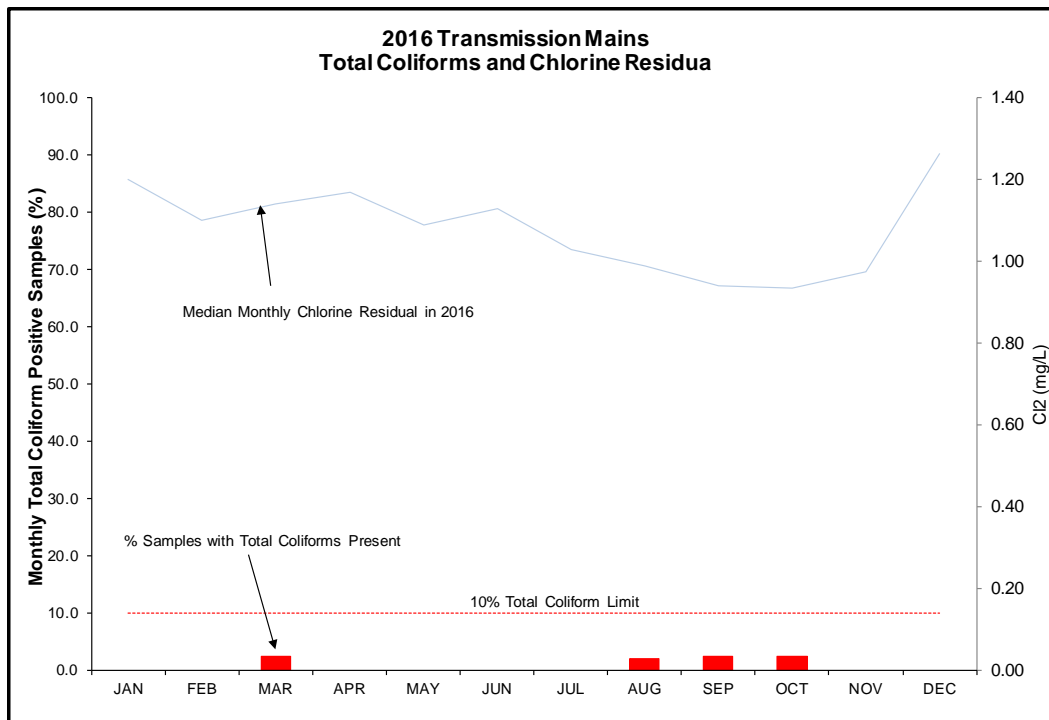
Figure 18 2016 Transmission Mains Total Coliforms and Chlorine Residual
