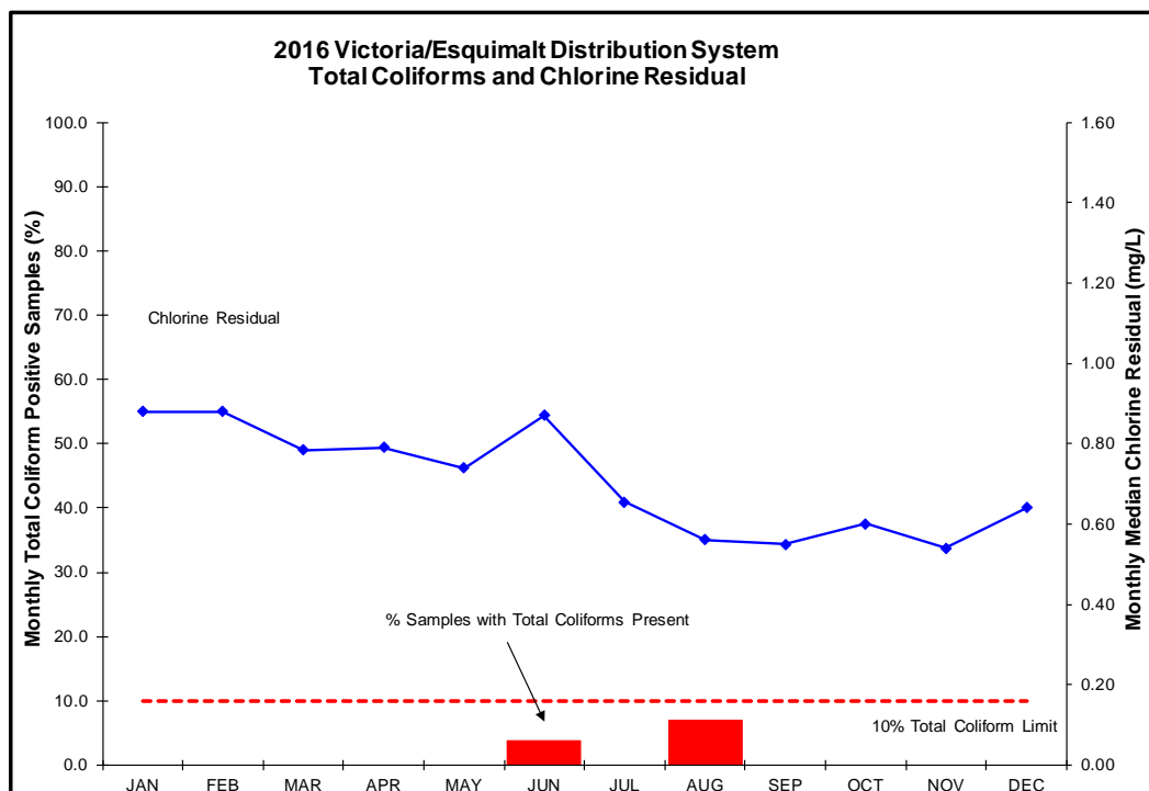
Figure 27 Victoria/Esquimalt Distribution System Total Coliforms and Chlorine Residuals in 2016
