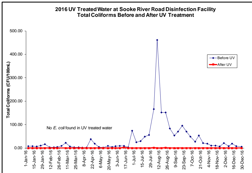
Figure 16 2016 UV Treated Water at Sooke River Road Disinfection Facility Total Coliforms Before and After UV Treatment
