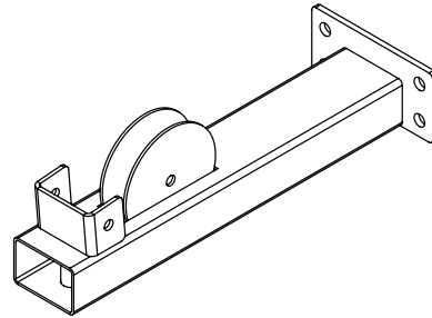
PART J - GUIDE POST , 1PCS.
