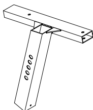
PART G -- SEAT FRAME, 1 PCS
