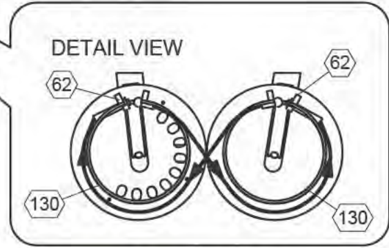
TURNPLATE CABLE (130)
