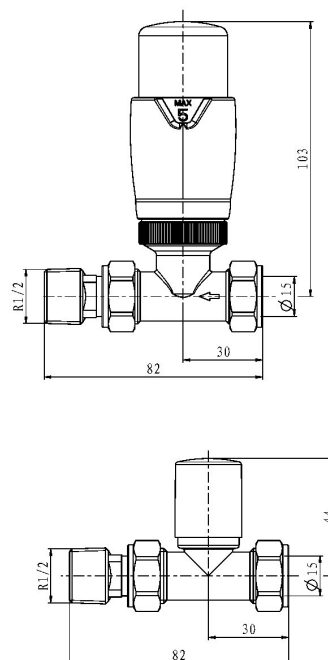
Dimensions (Measurements in mm)
